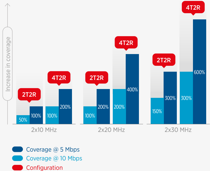
Figure 9: Impact of bandwidth and MIMO on 700 MHz band 4
