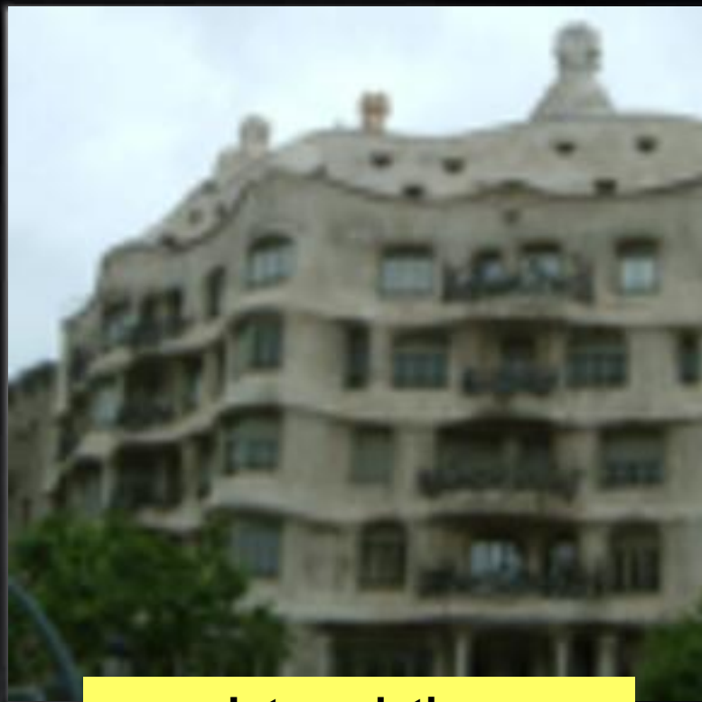
Interpolation
